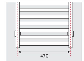
Pipe Centre Tappings (mm)
