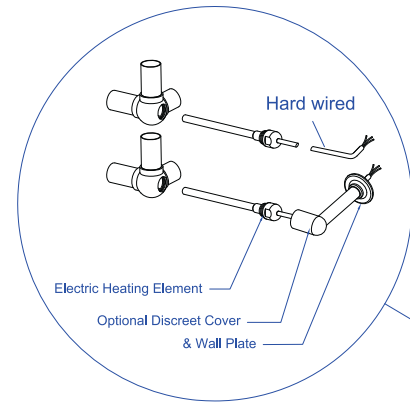
Heater Kit Assembly (UK)
