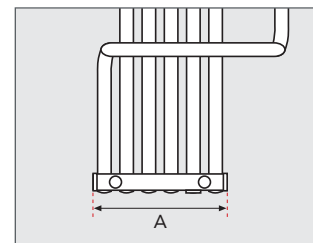
Pipe Centre Tappings (mm) (shows reverse of product)
