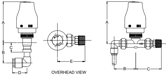
10/15mm TRV (90° Pushfit Elbow)
